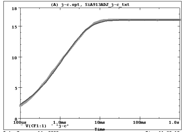
SiA913ADJ Filter j-c Temperature:27.0
