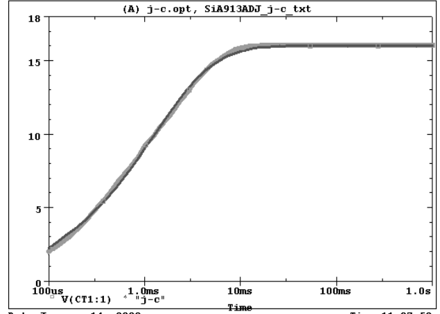
SiA913ADJ Tank j-c Temperature:27.0
