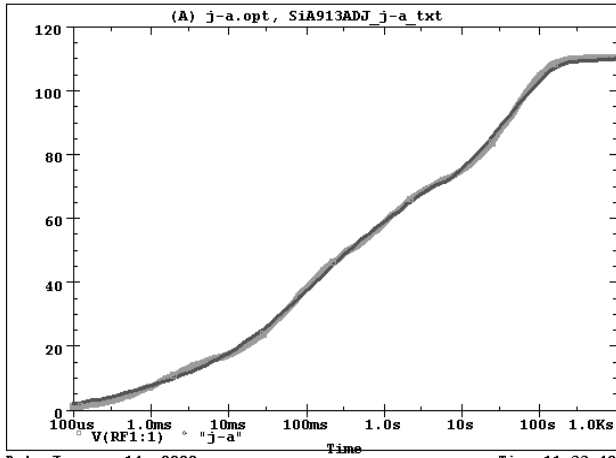
SiA913ADJ Filter j-a Temperature:27.0
