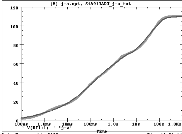
SiA913ADJ Tank j-a Temperature:27.0
